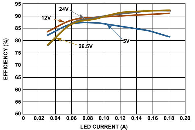
FIGURE 10. EFFICIENCY vs LED CURRENT AT LX FREQUENCY = 600kHz AT 25^{\circ}\text{C} vs V_{IN}
