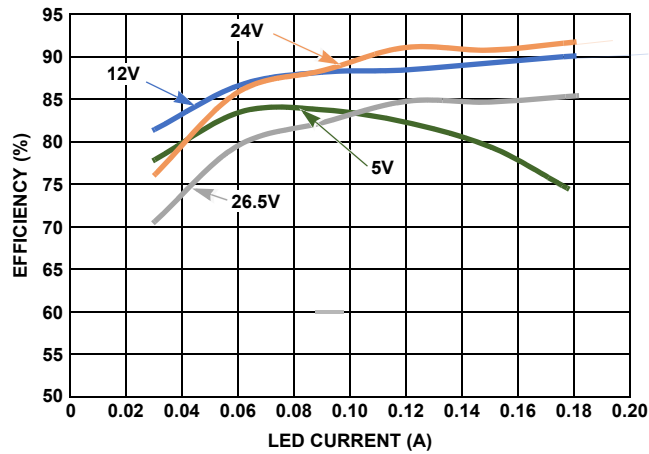
FIGURE 11. EFFICIENCY vs LED CURRENT AT LX FREQUENCY = 600kHz AT +105^{\circ}\text{C} vs V_{IN}
