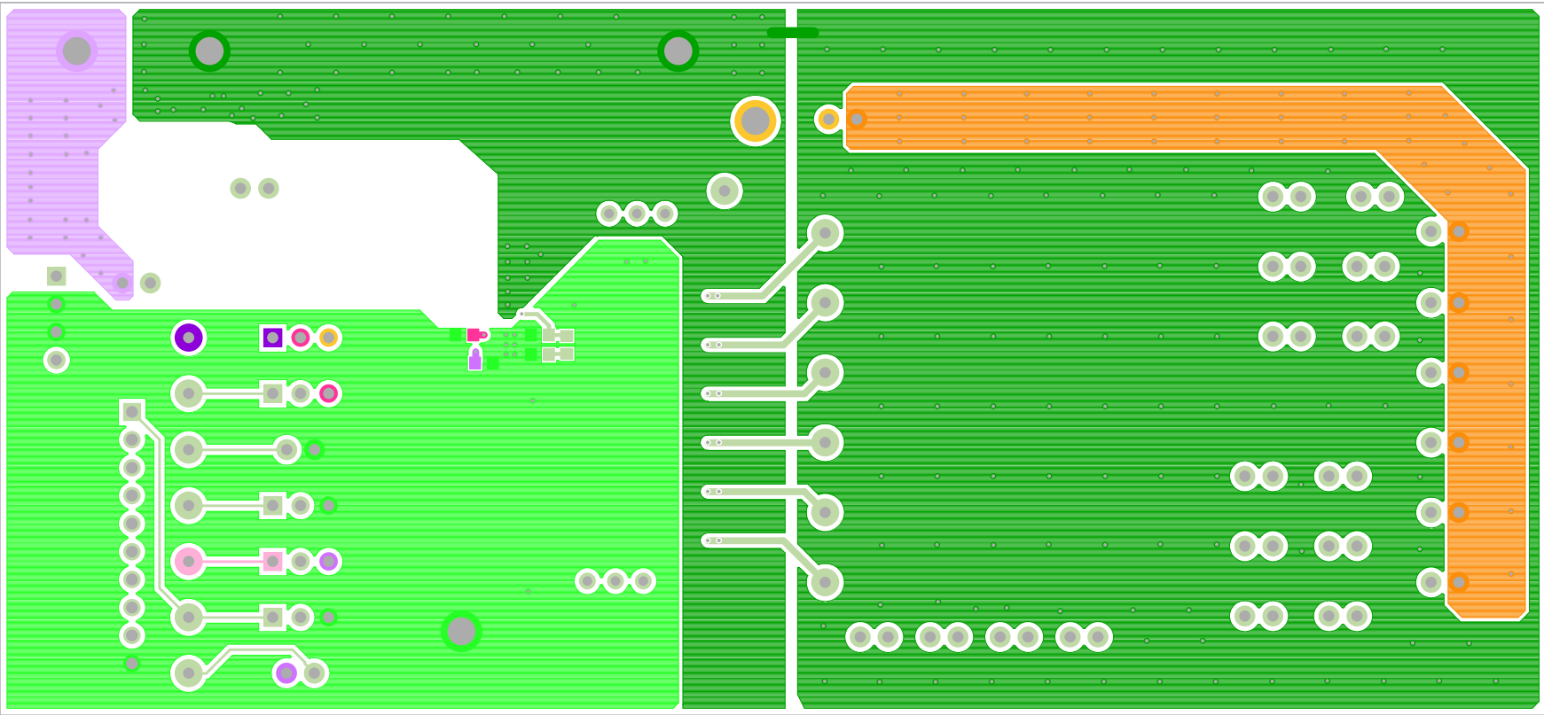
FIGURE 5. BOTTOM LAYER
