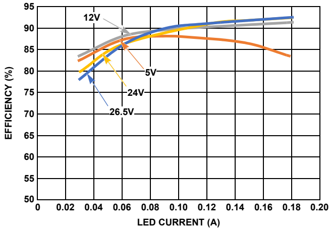
FIGURE 9. EFFICIENCY vs LED CURRENT AT LX FREQUENCY = 600kHz AT -40^{\circ}\text{C} vs V_{IN}
