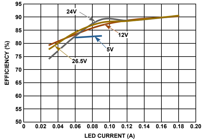
FIGURE 14. EFFICIENCY vs LED CURRENT AT LX FREQUENCY = 1.2MHz AT 25^{\circ}\text{C} vs V_{IN}
