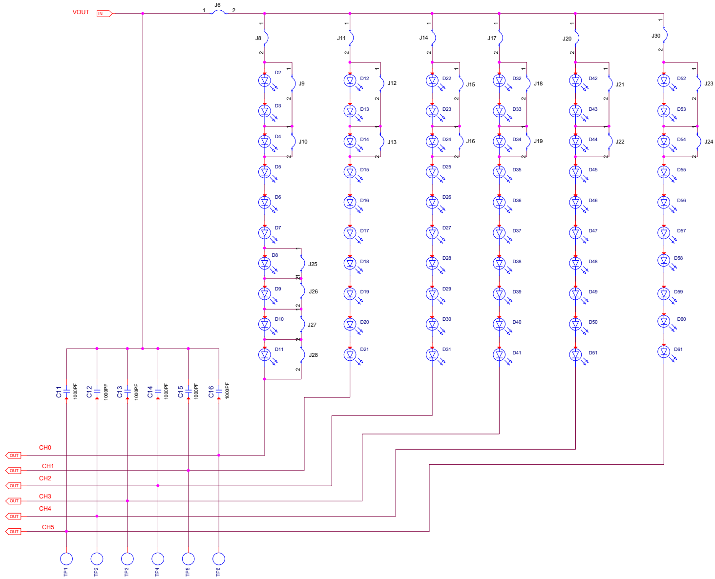
FIGURE 8. SCHEMATIC (PAGE 2)
